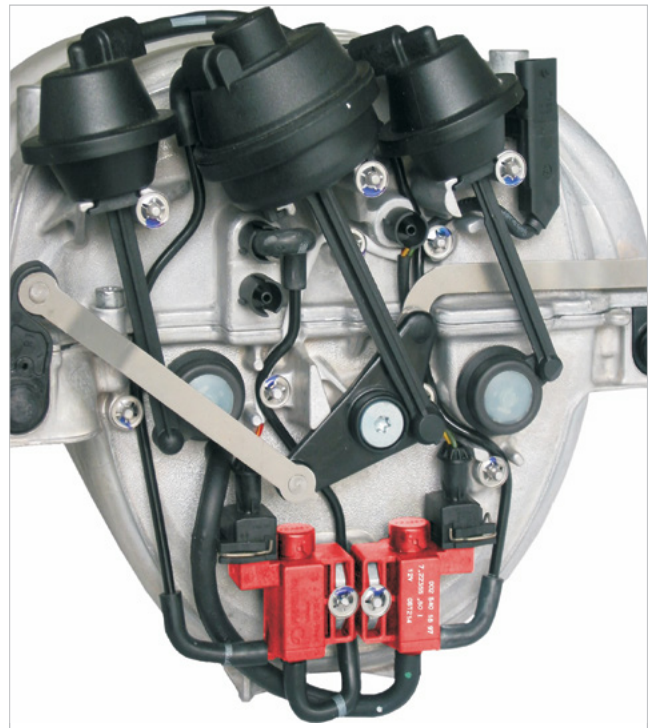
Application example: Intake manifold with electropneumatic valves (highlighted in red) as used in Mercedes-Benz C Class vehicles
